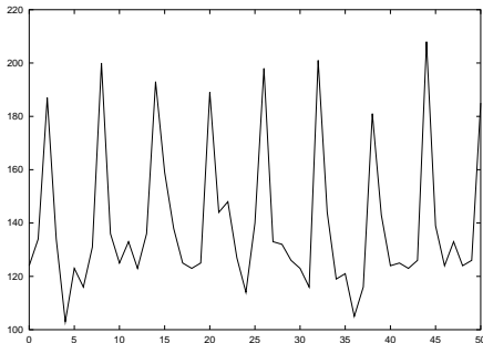
Fig. 3. Newspaper Sales per Day.
